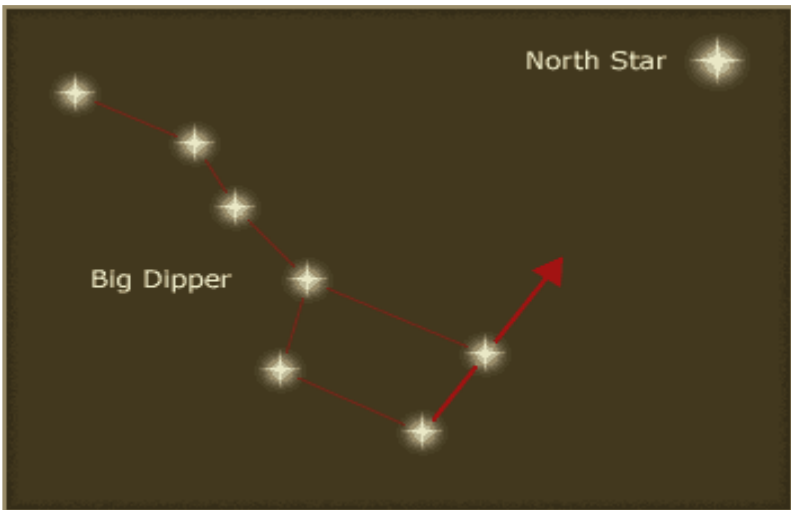
Figure: 1b The “Big dipper” pointing to the “North Star”
