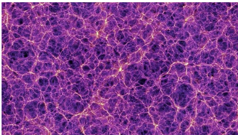
Figure: 7 A Swiss scientist's impression of the network that may be present in the universe as a result of the dark energy
