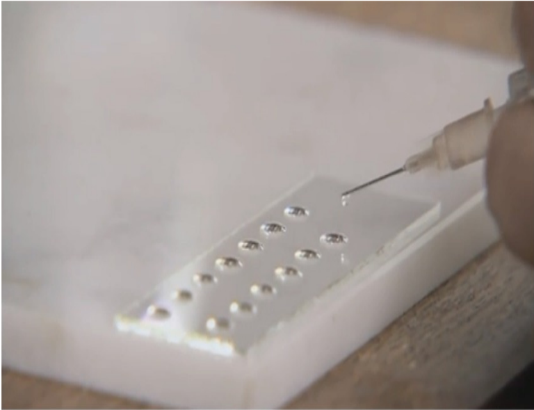
Figure: IX-a Showing the drops of water
