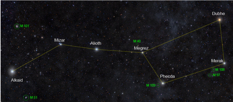
Figure: 1a The constellation “Big dipper” with its seven stars
